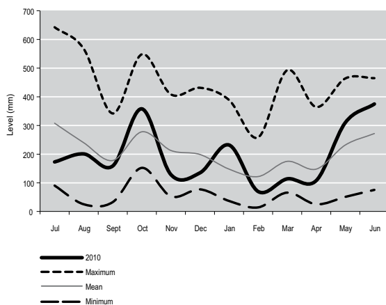
ORONGORONGO CATCHMENT RAINFALL (Orongorongo Swamp record 1980-2010)
