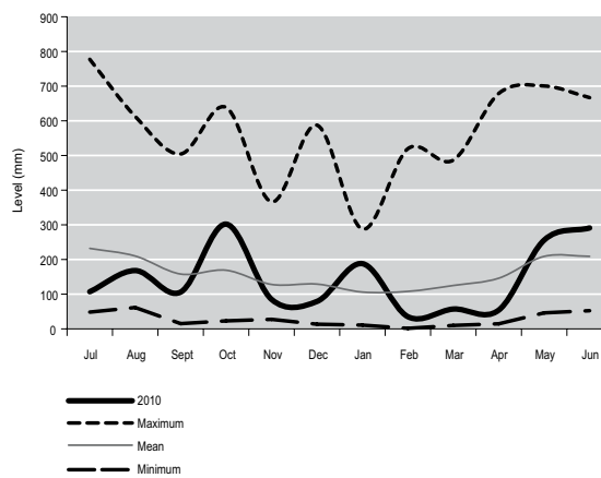
WAINUIOMATA CATCHMENT RAINFALL (Wainuiomata Reservoir record 1890-2010)
