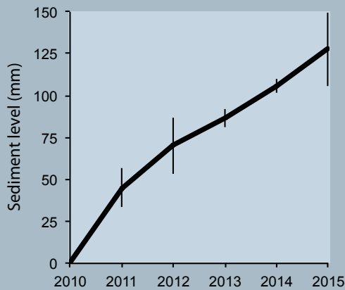
Figure 2. Change in mean sediment level over buried plates (+/- annual range), Waikanae Estuary, 2010 to 2015.
