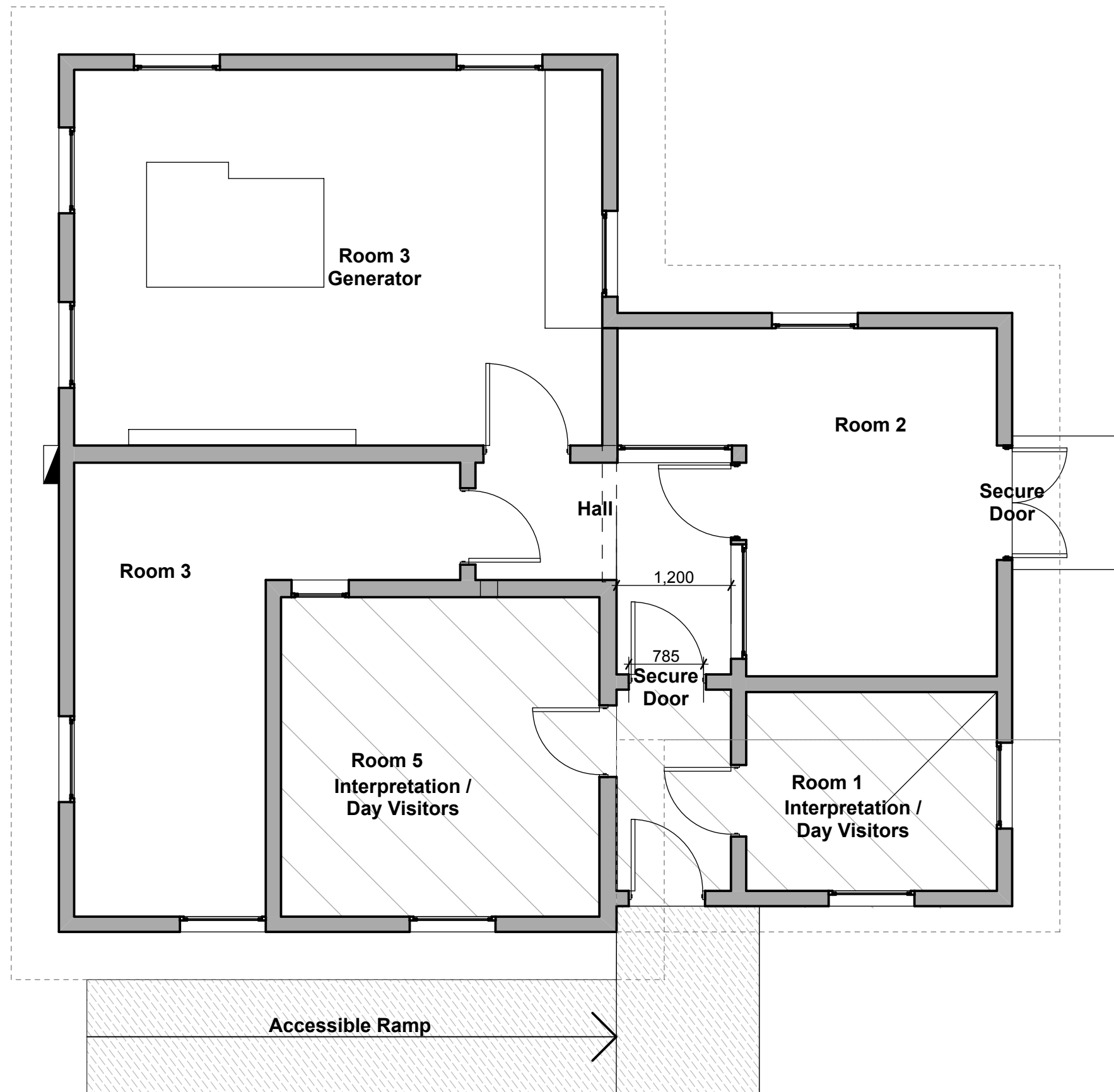
1 Power House Final Concept Plan Scale 1:50
