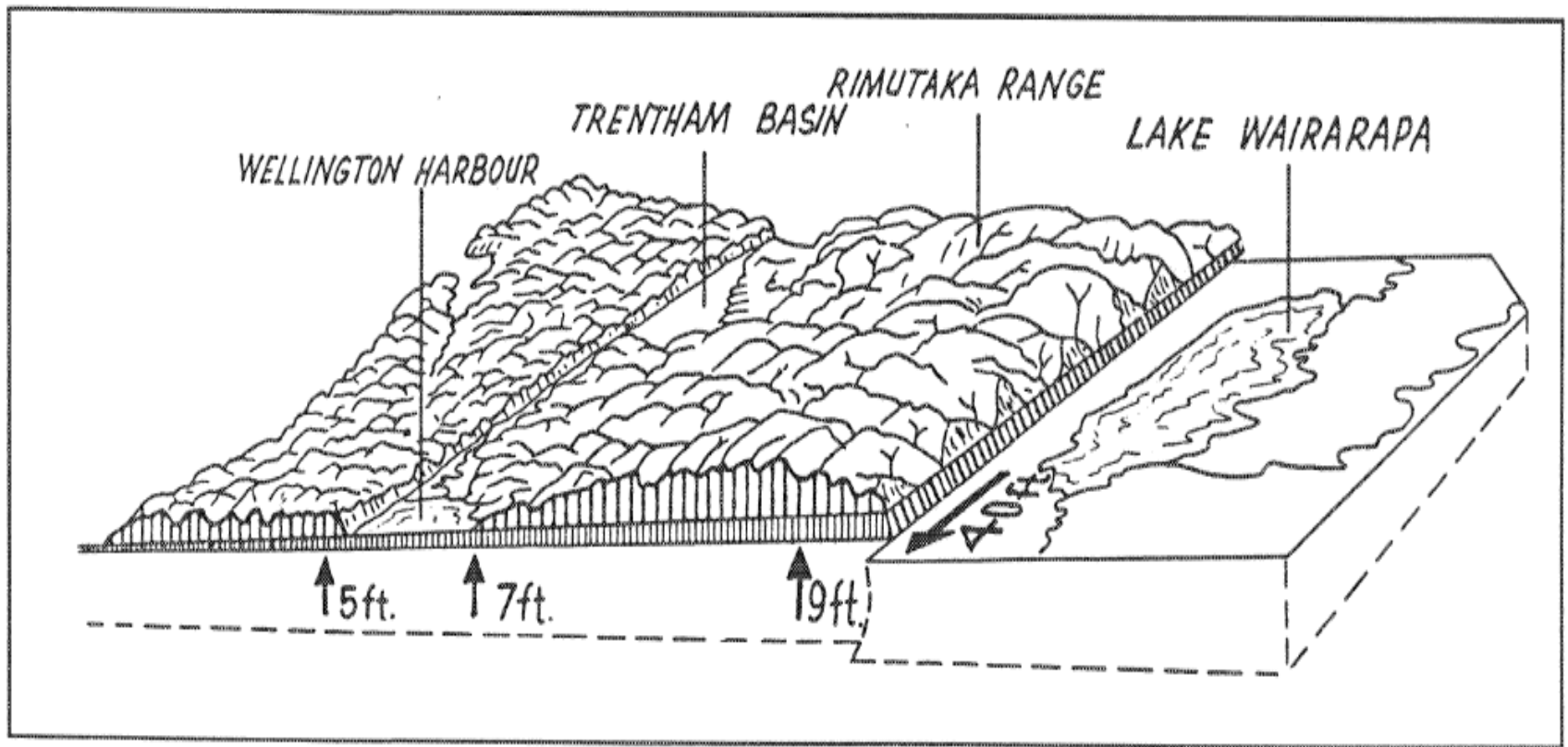
Fault movement, 1855 earthquake
