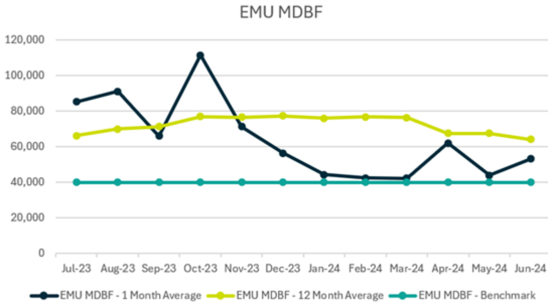
Figure 27: EMU reliability
